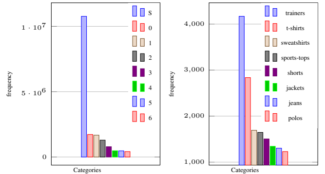
Fig. 2. Top 8 product categories appeared in the yoochoso and the second dataset respectively
