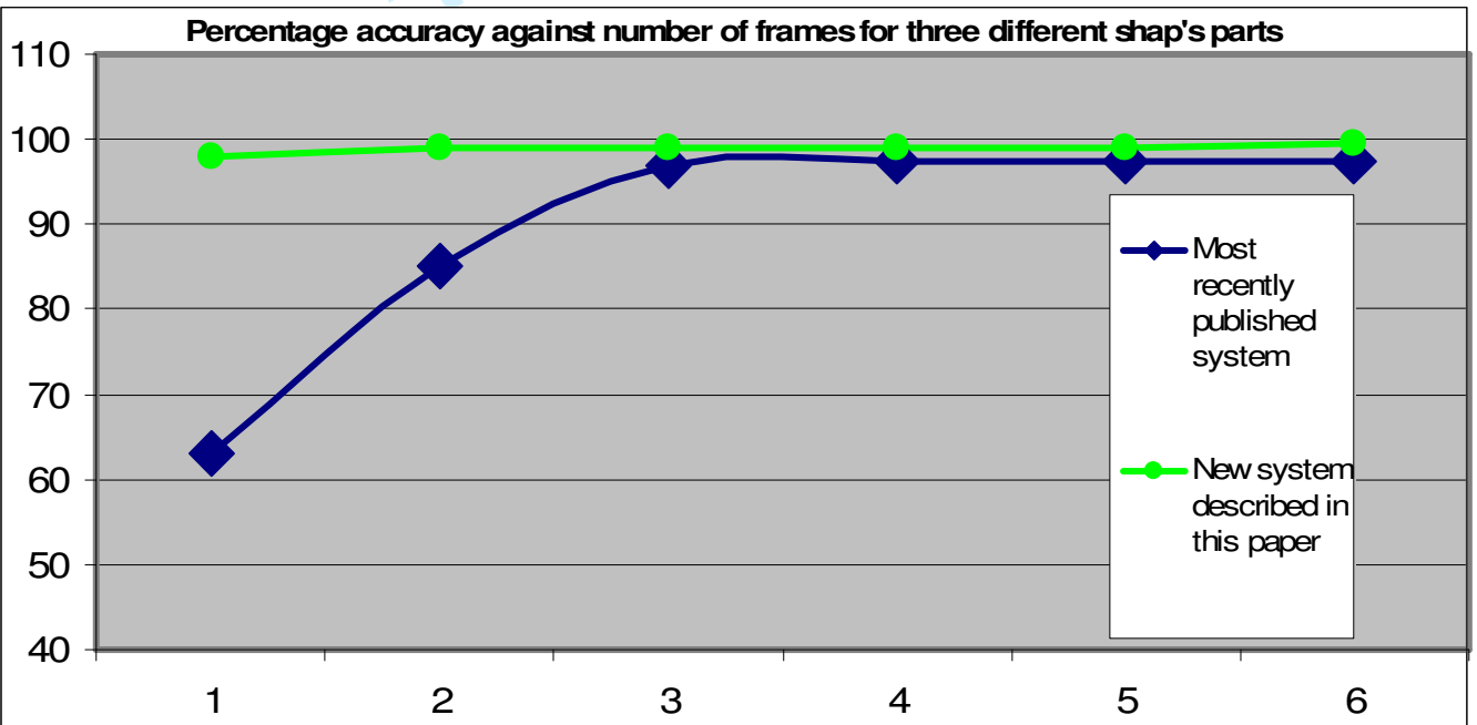
Figure 7 – Comparing the prototype system with the new system incorporating the corner finder.
