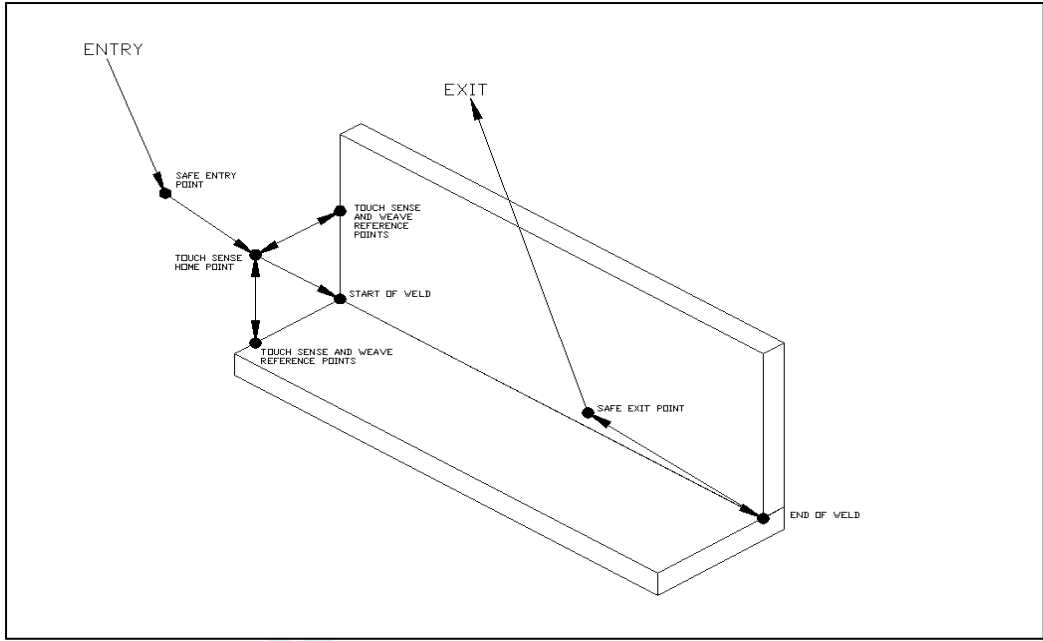
Figure 5 – End Effector Path Diagram
