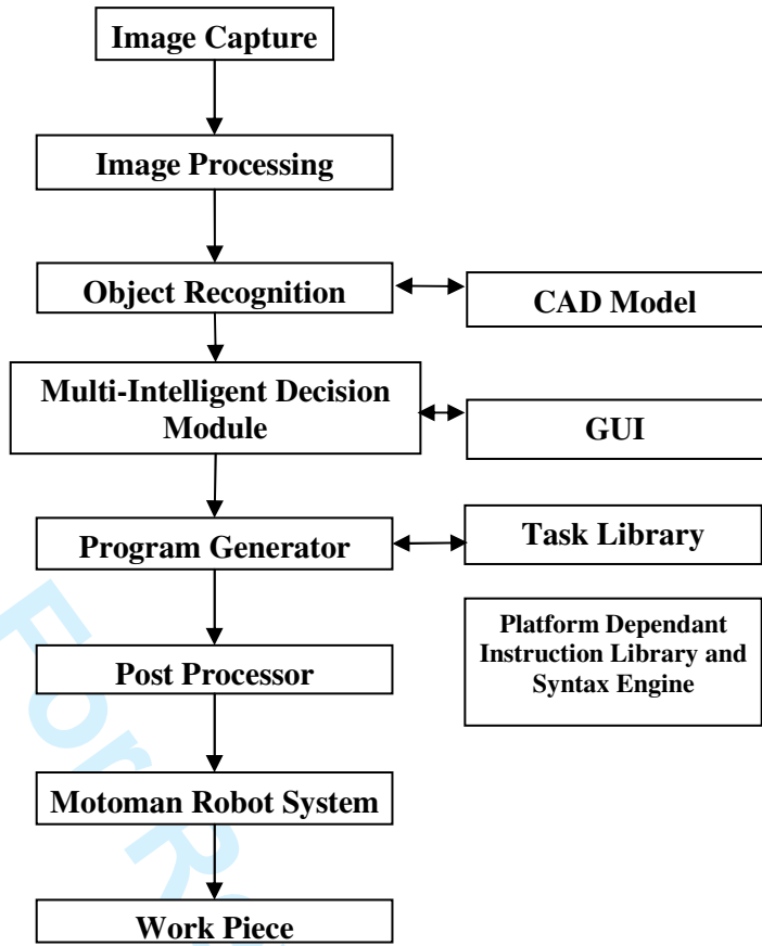
Figure 3 – Revised System Flow Diagram showing the inclusion of the computer aided design (CAD) model an the graphical user interface (GUI)
