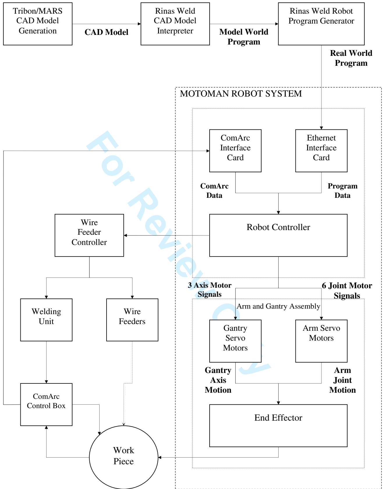
Figure 2 – Existing RinasWeld / Motoman System
