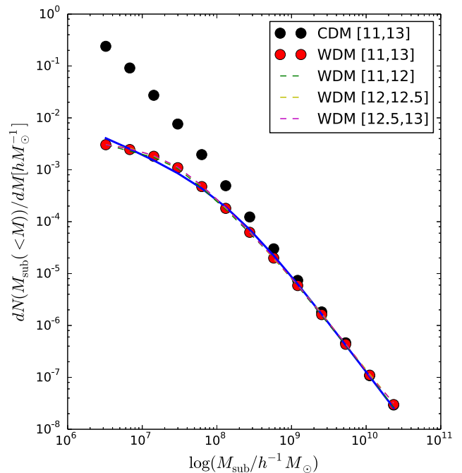
Figure 1. The differential SHMF for host haloes of different mass. The solid black (COCO-COLD) and red (COCO-WARM) points show the SHMF for host haloes with mass in range [10^{11} h^{-1} M_\odot, 10^{13} h^{-1} M_\odot] . The dashed lines show the mass function for haloes in different mass ranges in COCO-WARM. We scale the dashed lines to match the red solid points (by requiring the average amplitude of different curves to be the same), so that one can compare the shape of the SHMFs in COCO-WARM. The blue line shows the fit to the SHMF in COCO-WARM.
