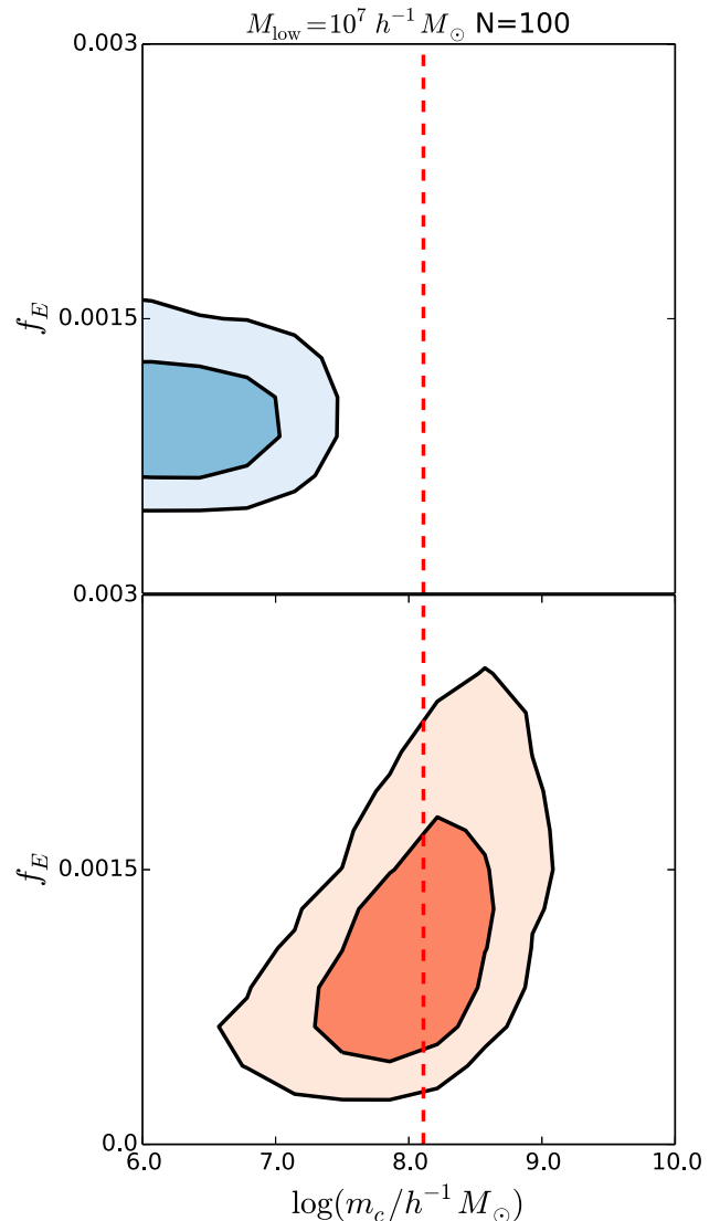
Figure 5. The 2D posterior probability distribution of f_E and m_c , assuming N = 100, M_{\text{low}} = 10^7 h^{-1} M_\odot . The lower panel shows the results with input model of COCO-WARM (red), and the upper panel shows the results with input mode of COCO-COLD (blue). The vertical dashed line shows the m_c value of the COCO-WARM simulation.
