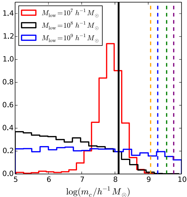
Figure 4. The marginalized 1D probability distribution of m_c for different detection mass limits with N = 100 . The mock systems are generated using COCO-WDM SHMF. The vertical black solid line shows the m_c value of the COCO-WARM simulation. The coloured dashed lines from left to right show the m_c values of WDM models with particle masses m_{\text{WDM}} = 2.28, 1.95, 1.59, 1.41 keV, respectively.
