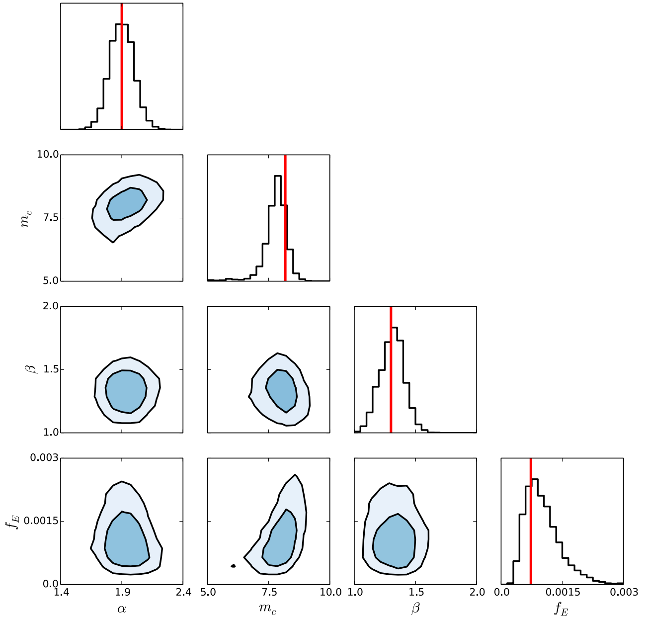
Figure 2. Parameter constraints from 100 mock systems constructed using parameters appropriate to the COCO-WARM simulation. The contours show the 68 and 95 per cent confidence levels for the 2D posterior probability distribution of the model parameters. The histograms at the end of each row show the marginalized 1D posterior probability distribution for each model parameter. The red vertical lines show the input values of each model parameter. The assumed detection limit is M_{\text{low}} = 10^7 h^{-1} M_{\odot} .
