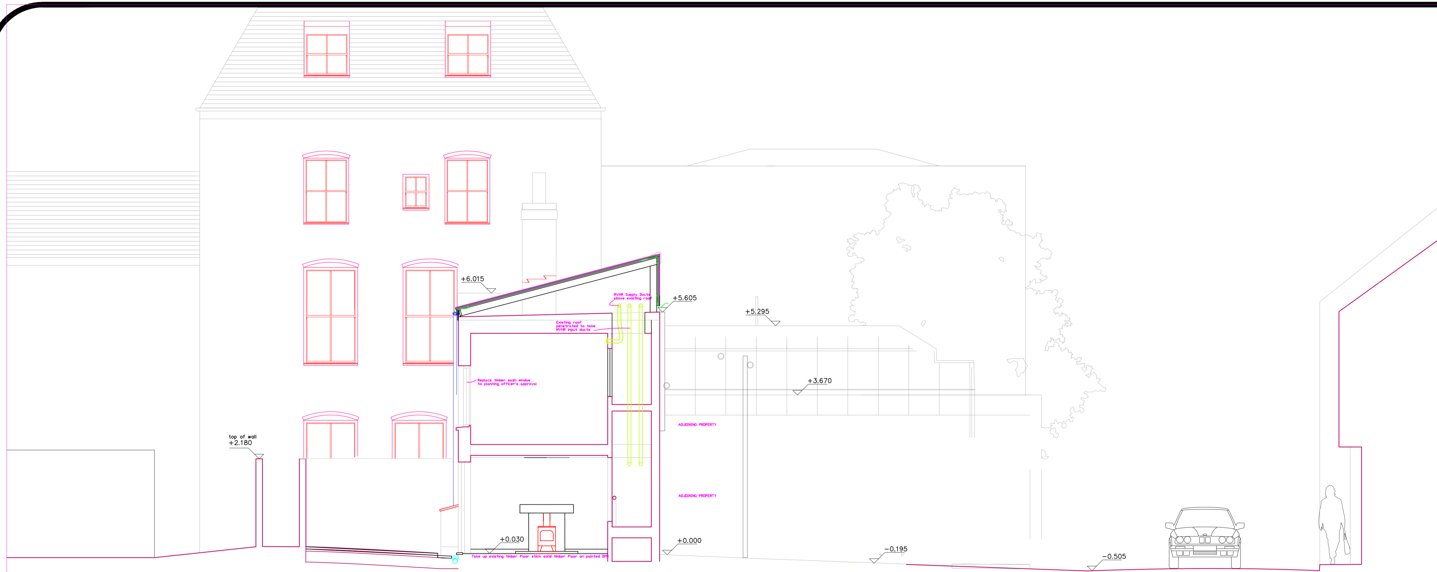
SECTION CC
